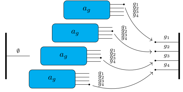
Figure 3: A POCL plan with four identical actions executing at once.
