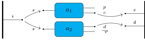
Figure 2: A POCL plan where the order between a_1 and a_2 is unconstrained. Arrows depict causal links and implied ordering constraints are not shown.
